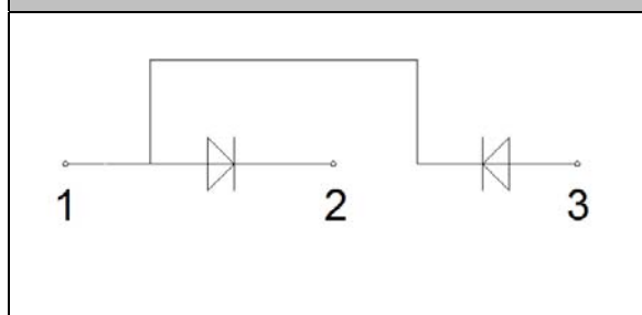
Circuit
